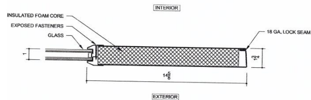
3 DOOR SECTION SCALE: 3/8"=1'-0"
